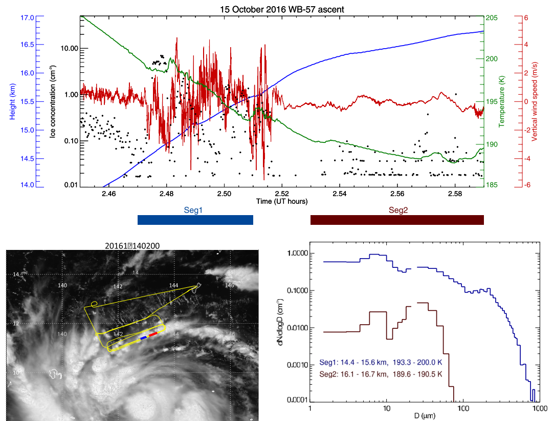
Figure 2. Top panel: Time series of Pacific Oxidants, Sulfur, Ice, Dehydration, and cONvection (POSIDON) in situ measurements during the WB-57 transect through a band of convection emanating from tropical cyclone Haima: aircraft altitude (blue), temperature (green), vertical wind speed (red), and ice concentration (black dots). Lower left: satellite image showing the flight segment along a band of convection. Lower right: Size distributions averaged over the two different flight segments shown underneath the time series plot in the top panel.
